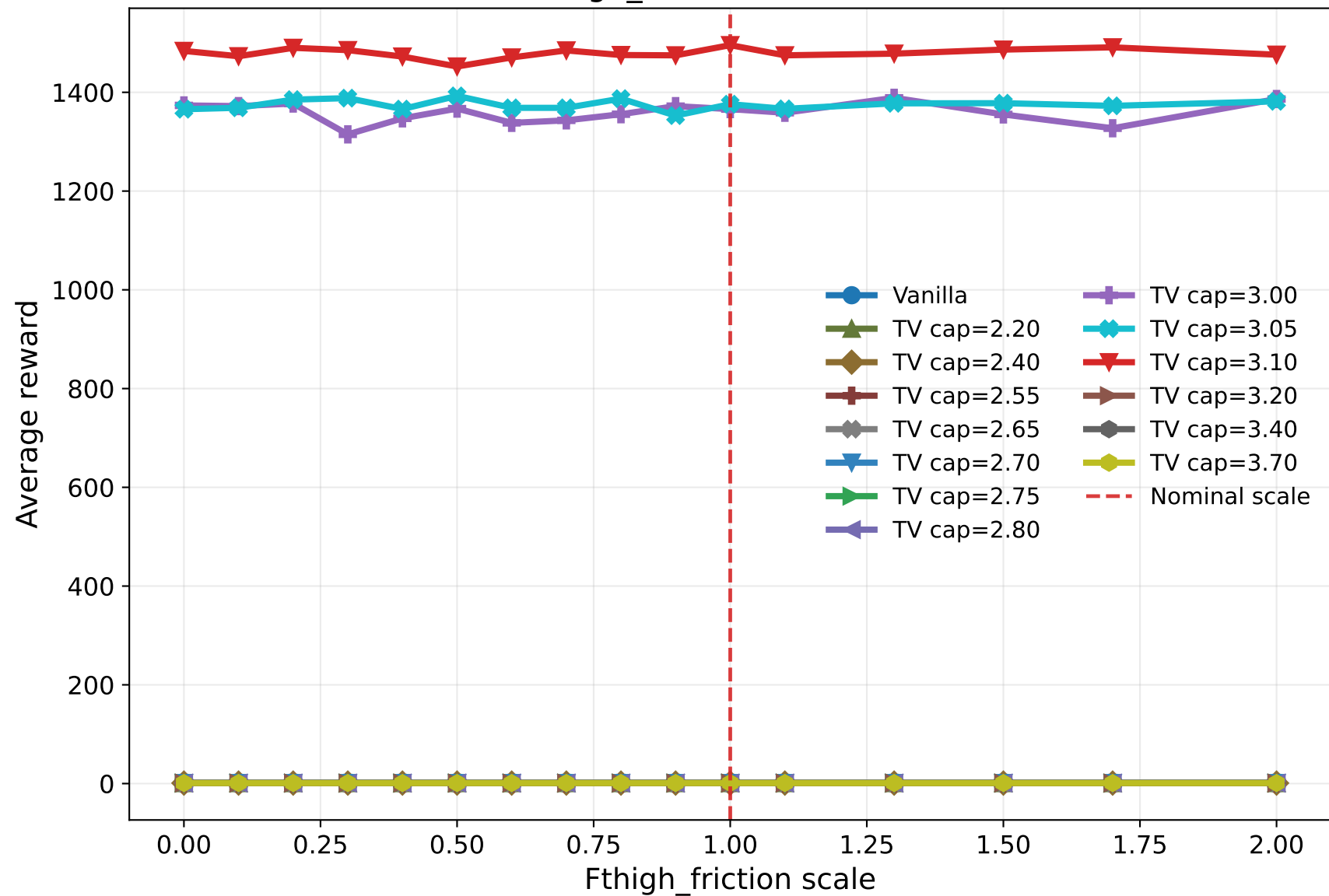
Fthigh_friction robustness
